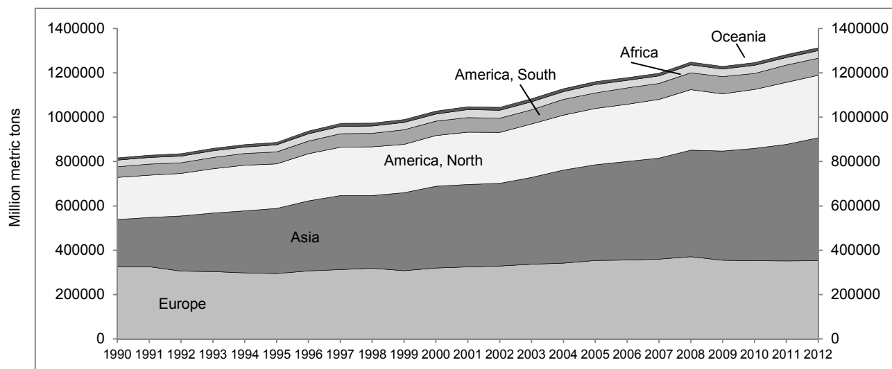
Figure 57: Production of gas/diesel oil by region, 1990-2012
