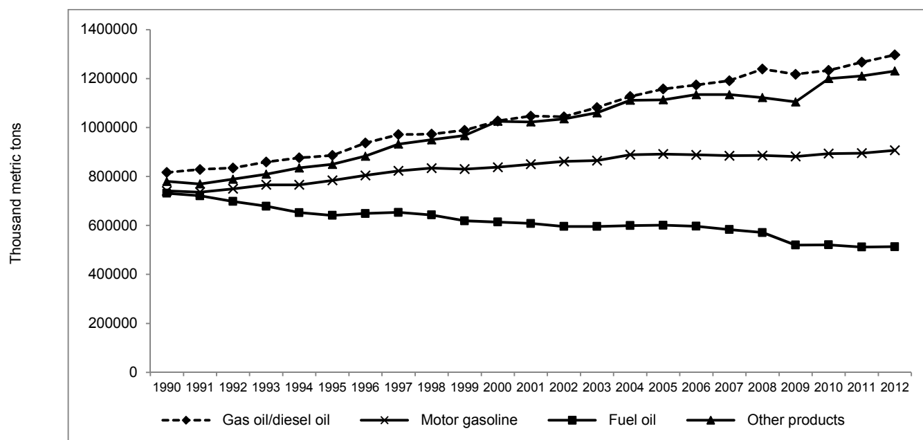
Figure 64: Production of selected oil products from refineries, 1990-2012
