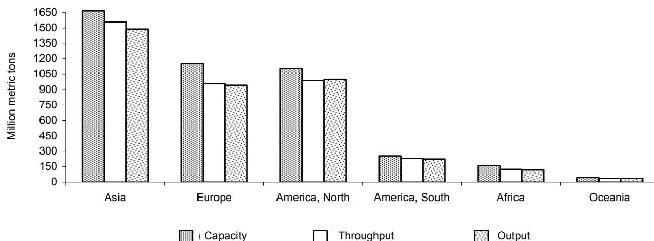
Figure 44: Refinery distillation capacity, throughput and output, by region, in 2010
