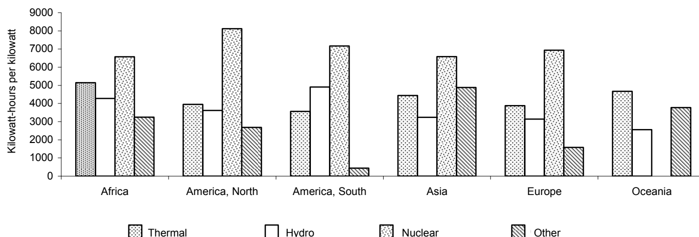
Figure 82: Utilization of installed electric generating capacity, by region, by type, in 2010
