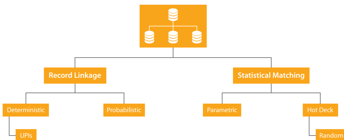
Figure 4.2: Data integration
