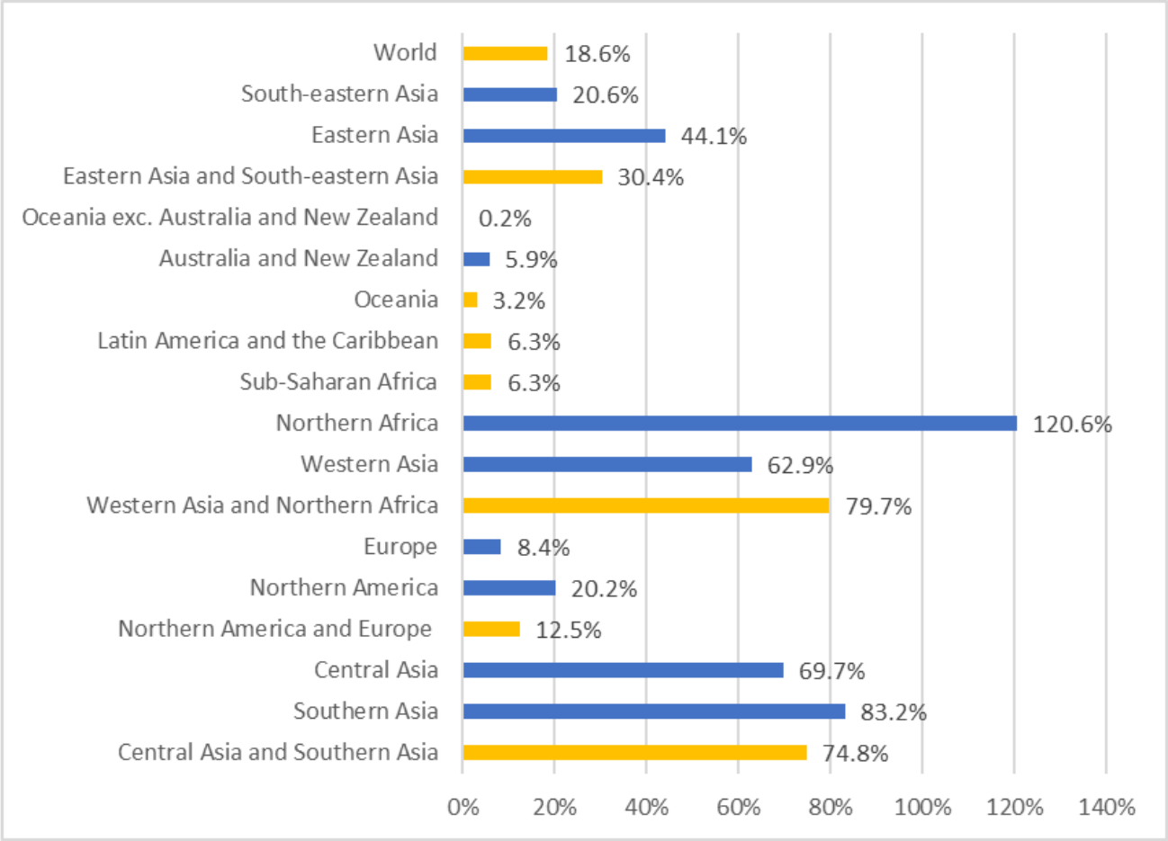
Figure 2: Level of water stress by SDG region and sub-region (2021)
